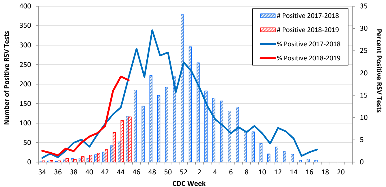
Figure 3. Number and Percent Positive RSV Rapid Antigen and PCR Tests by Week, NREVSS Surveillance Data, North Texas: August 25, 2017 – November 10, 2018
