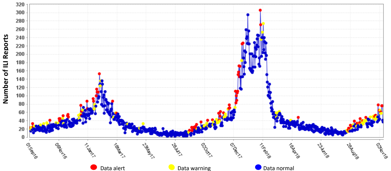
Figure 2. Syndromic Surveillance of Emergency Department Visits for Influenza-like Illness (ILI), Dallas County: September 1, 2016 – November 10, 2018
