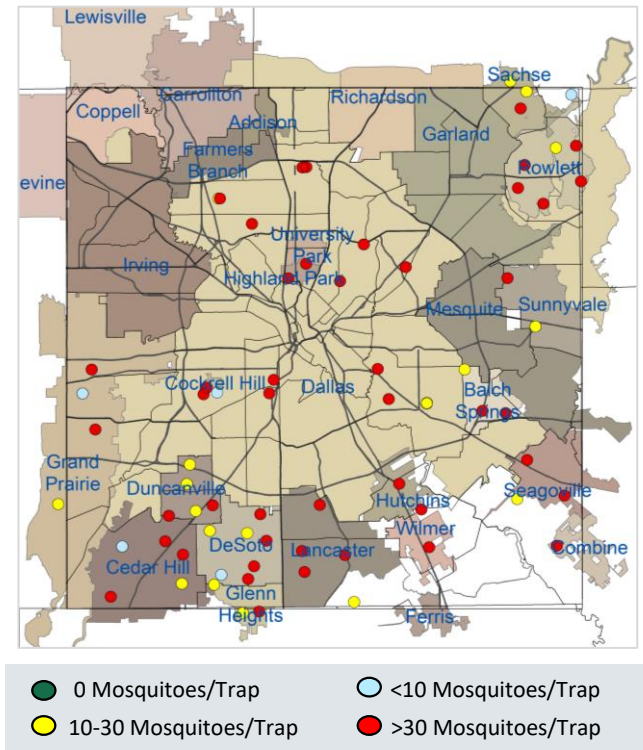
Figure 9: BG-Sentinel Trap Counts of Female Aedes aegypti and Aedes albopictus During 2018: Weeks 13 through 41
