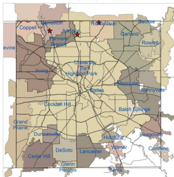
Figure 2: Cumulative WNV Positive Mosquito Traps Collected: Weeks 1-21 (N=3 † )
