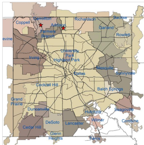
Figure 3: WNV Positive Mosquito Traps Collected During 2019: Weeks 20 and 21* (N=2)
