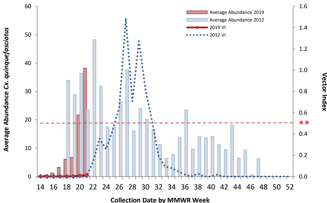
Figure 5: Average Numbers of Female Cx. quinquefasciatus per Trap-night and WNV Vector Index by Week: 2012 Season and 2019 Season (through Week 21*)
