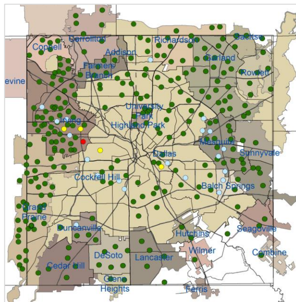
Figure 4: Trap Counts of Female Cx. quinquefasciatus from 2019 Season: Weeks 1-21*
