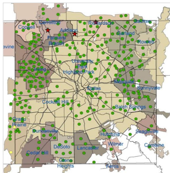
Figure 1: All WNV Negative and Positive Mosquito Traps Collected During 2019: Weeks 1-21 (N=1,743)
