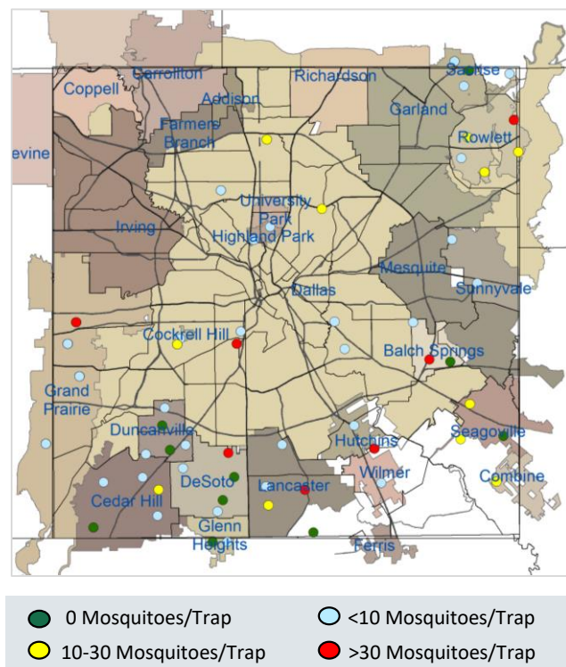
Figure 9: BG-Sentinel Trap Counts of Female Aedes aegypti and Aedes albopictus during 2019: Weeks 14 through 21 †
