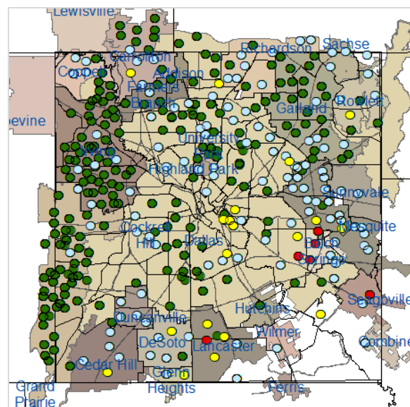
Figure 4: Trap Counts of Female Cx. quinquefasciatus from 2021 Season: Weeks 1-33*
