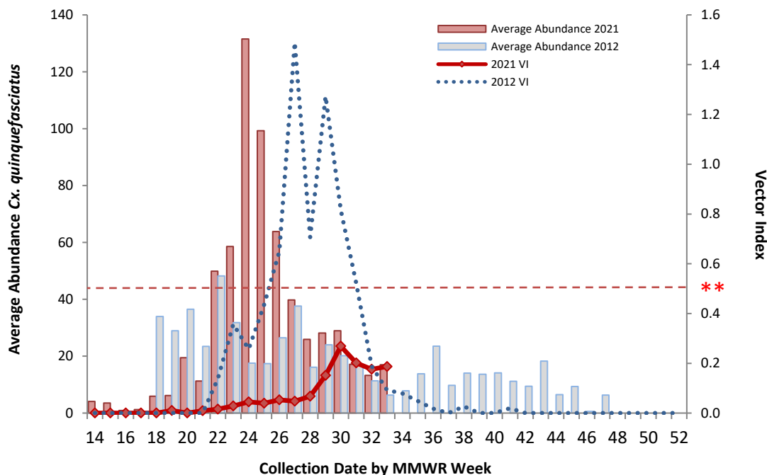
Figure 5: Average Numbers of Female Cx. quinquefasciatus per Trap-night and WNV Vector Index by Week: 2012 Season and 2021 Season (through Week 33*)
