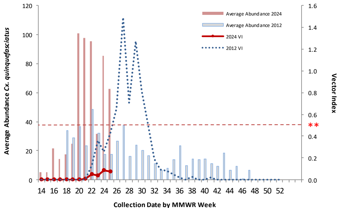
Figure 5: Average Numbers of Female Cx. quinquefasciatus per Trap-night and WNV Vector Index by Week: 2012 Season and 2024 Season (through Week 25*)
