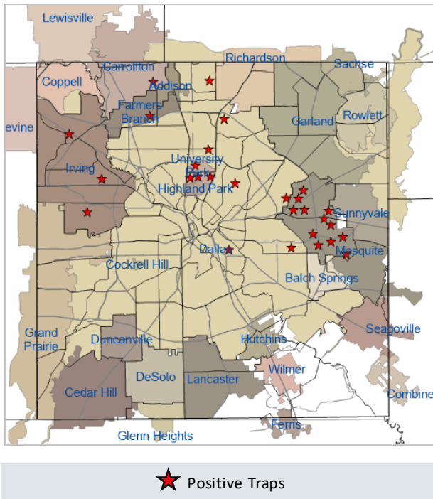
Figure 3: WNV Positive Mosquito Traps Collected During 2024: Weeks 24 and 25* (N=31)
