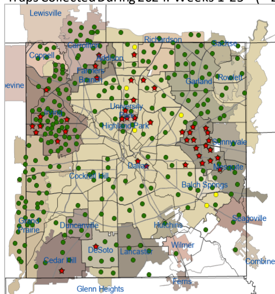
Figure 1: All WNV Negative and Positive Mosquito Traps Collected During 2024: Weeks 1-25* (= 2,051)
