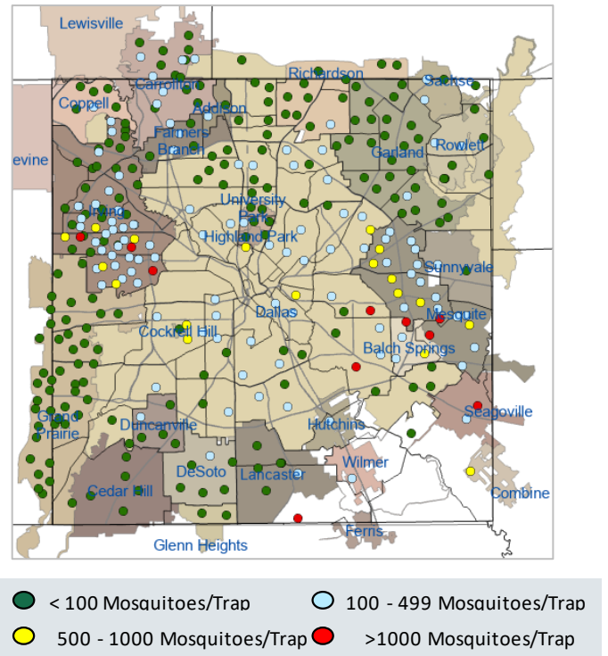
Figure 4: Trap Counts of Female Cx. quinquefasciatus from 2024 Season: Weeks 1-25*
