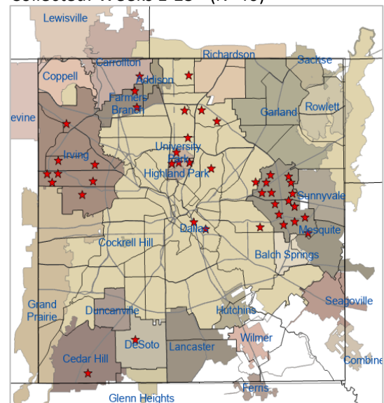
Figure 2: Cumulative WNV Positive Mosquito Traps Collected: Weeks 1-25* (N=46)
