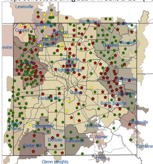
Figure 1: All WNV Negative and Positive Mosquito Traps Collected During 2024: Weeks 1-28* (= 2,648)
