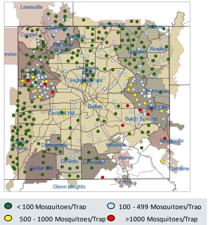
Figure 4: Trap Counts of Female Cx. quinquefasciatus from 2024 Season: Weeks 1-27*
