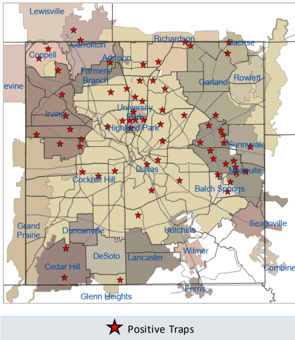
Figure 3: WNV Positive Mosquito Traps Collected During 2024: Weeks 26 and 27* (N=70)
