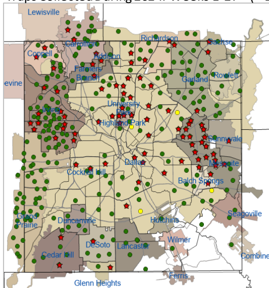
Figure 1: All WNV Negative and Positive Mosquito Traps Collected During 2024: Weeks 1-27* (= 2,423)
