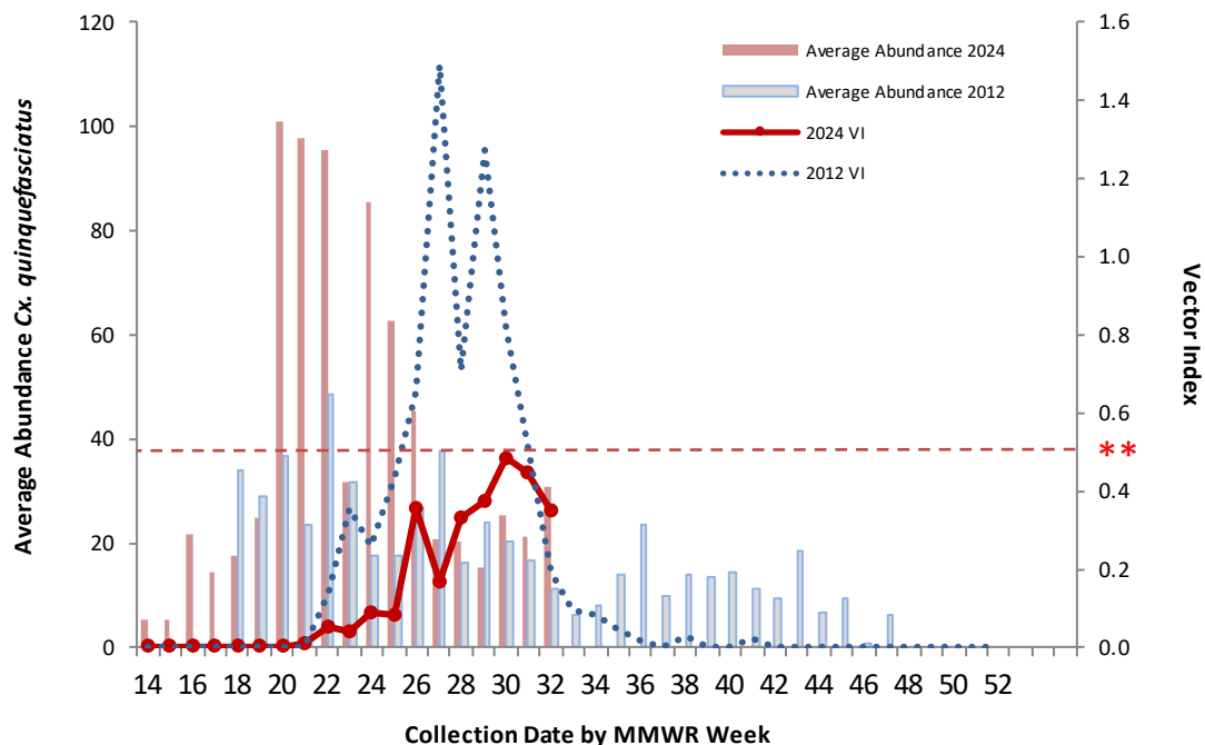
Figure 5: Average Numbers of Female Cx. quinquefasciatus per Trap-night and WNV Vector Index by Week: 2012 Season and 2024 Season (through Week 32*)
