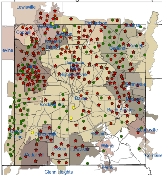
Figure 1: All WNV Negative and Positive Mosquito Traps Collected During 2024: Weeks 1-32* (= 3,583)
