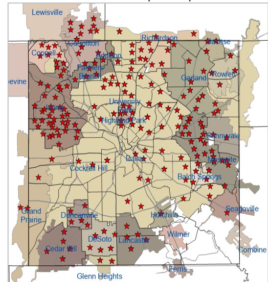
Figure 2: Cumulative WNV Positive Mosquito Traps Collected: Weeks 1-32* (N=433)
