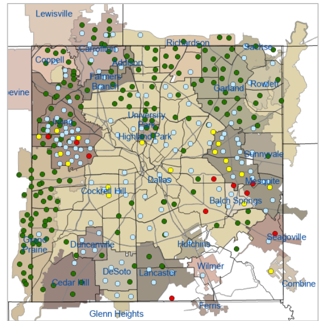
Figure 4: Trap Counts of Female Cx. quinquefasciatus from 2024 Season: Weeks 1-32*
