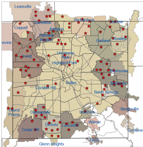
Figure 3: WNV Positive Mosquito Traps Collected During 2024: Weeks 31 and 32* (N=113)
