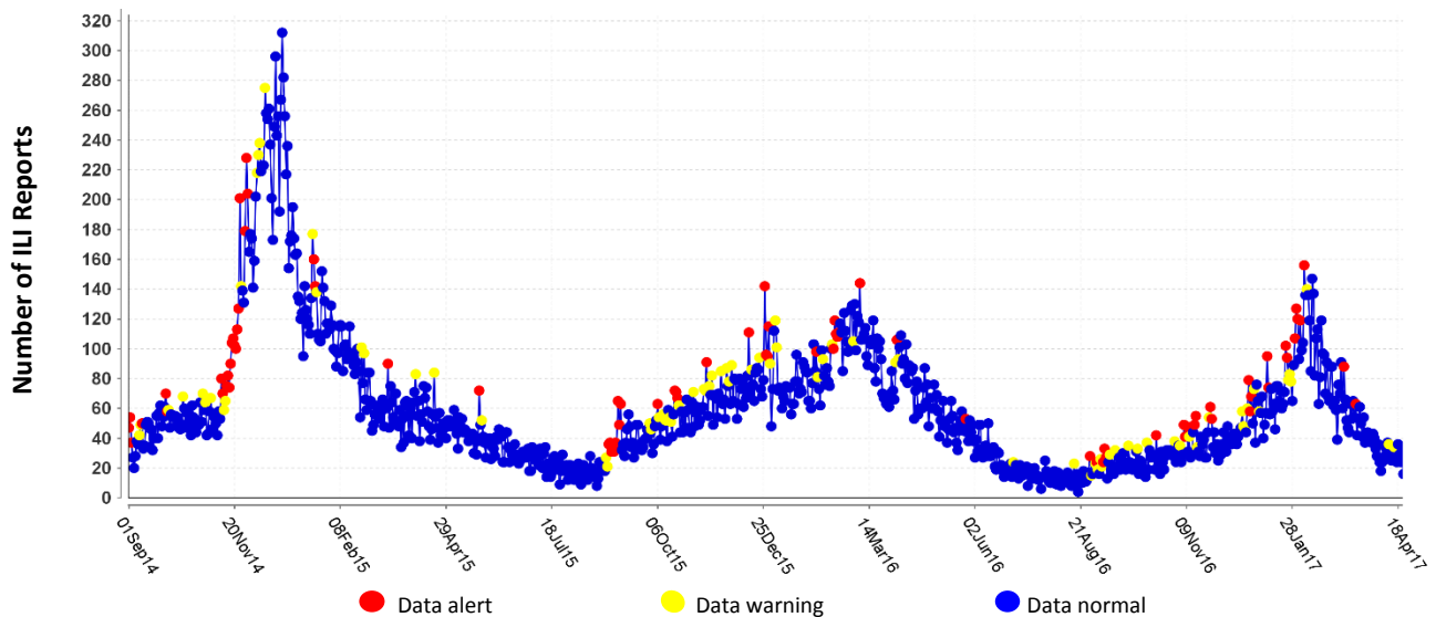
Figure 4. Syndromic Surveillance of Emergency Department Visits for Influenza-like Illness (ILI), Dallas County: September 1, 2014 – April 22, 2017
