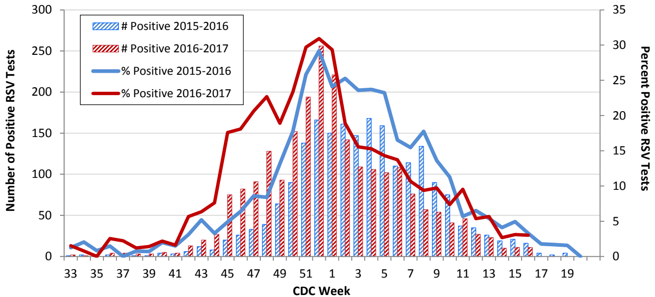
Figure 7. Number and Percent Positive RSV Rapid Antigen and PCR Tests by Week, NREVSS Surveillance Data, North Texas: August 22, 2015 – April 22, 2017
