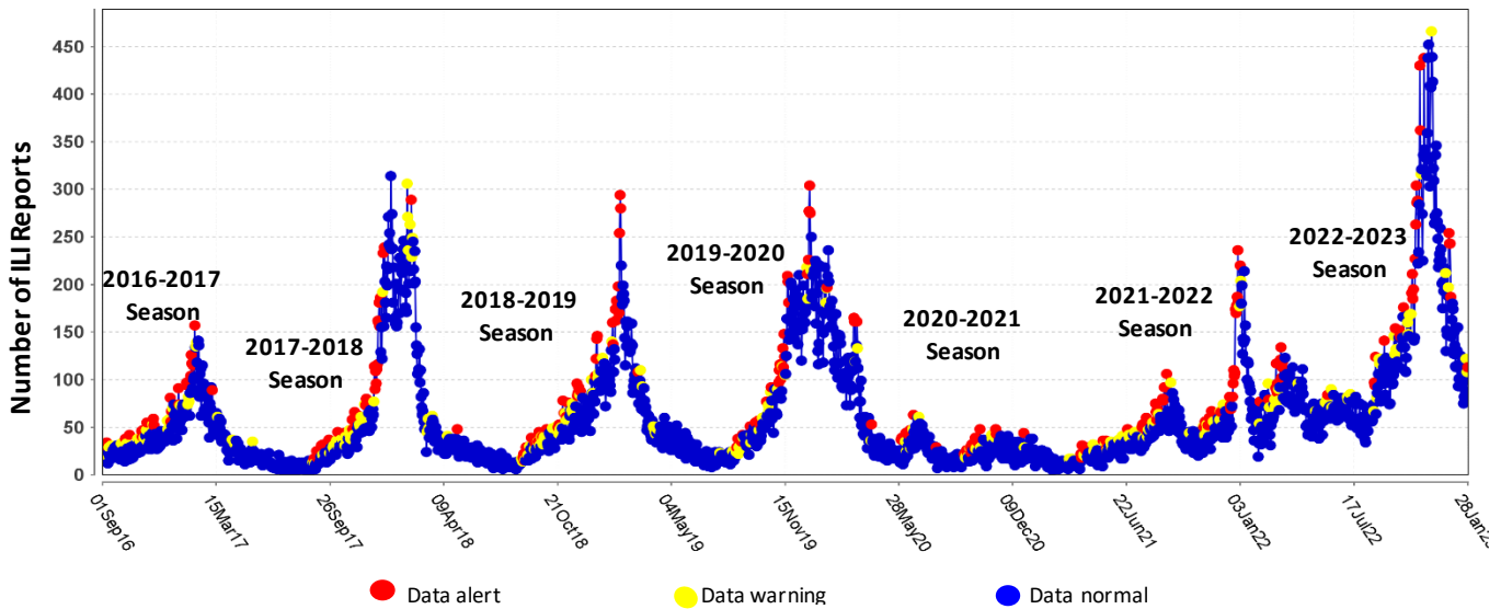
Figure 3. Syndromic Surveillance of Emergency Department Visits for Influenza-like Illness (ILI), Dallas County: September 1, 2016 – January 28, 2023
